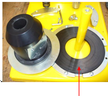
Plastic friction disk FS3.2303 (less tension)
